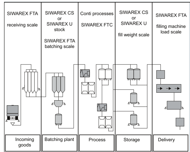
Applications of SIWAREX weighing technology in the production process
