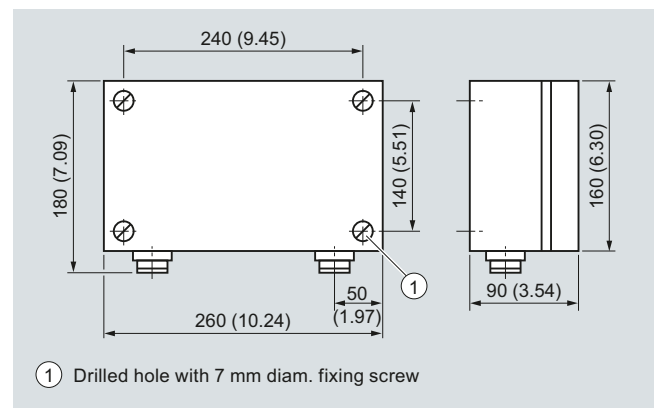
SIWAREX Pi, Ex-Interface, dimensions in mm (inch)
